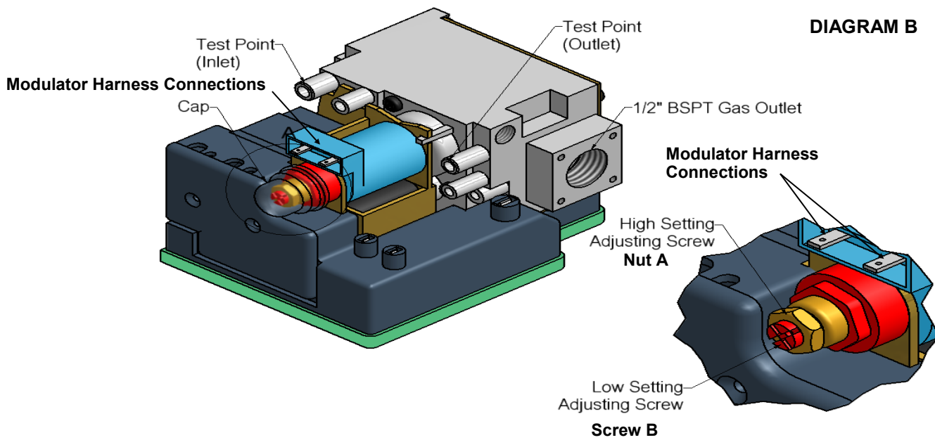
DIAGRAM B ( SHOWING CONTROL VALVE WITH TEST POINTS AND ADJUSTING SCREW ).
